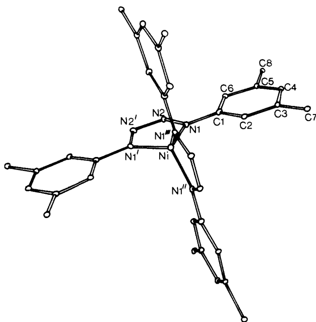
Figure 2. The structure of [(3,5-Me 2 C 6 H 3 N 4 C 6 H 3 Me 2 -3,5) 2 Ni]. For relevant bond distances and angles, see ref 10.
